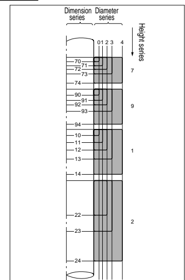
Fig. 5.6 Dimension series for thrust bearings
