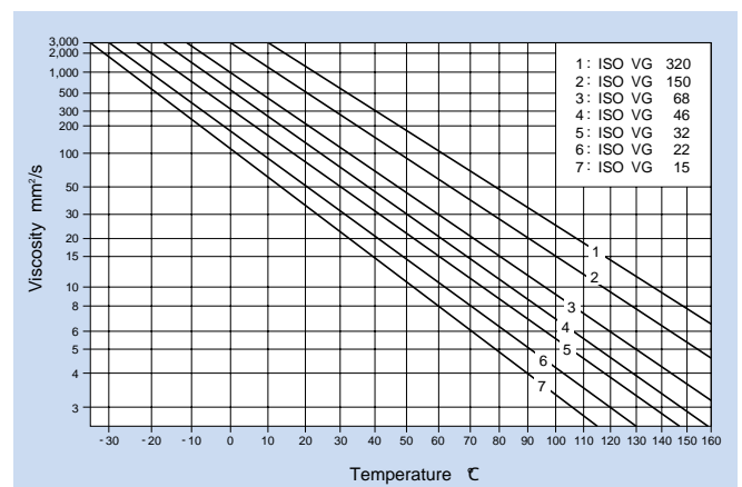
Fig. 11.5 Relation between lubricating oil viscosity and temperature
